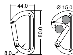
STRAIGHT GATE
